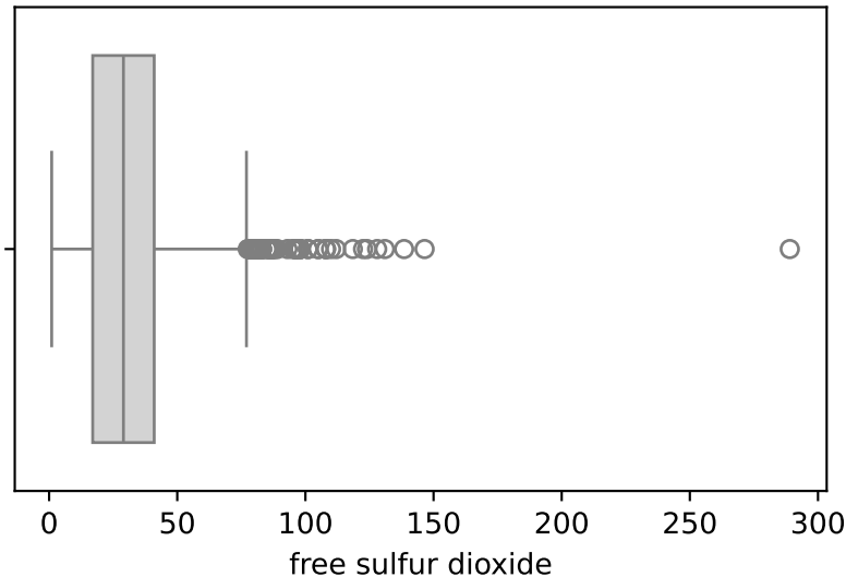
Box-plot Incondicional - free sulfur dioxide
